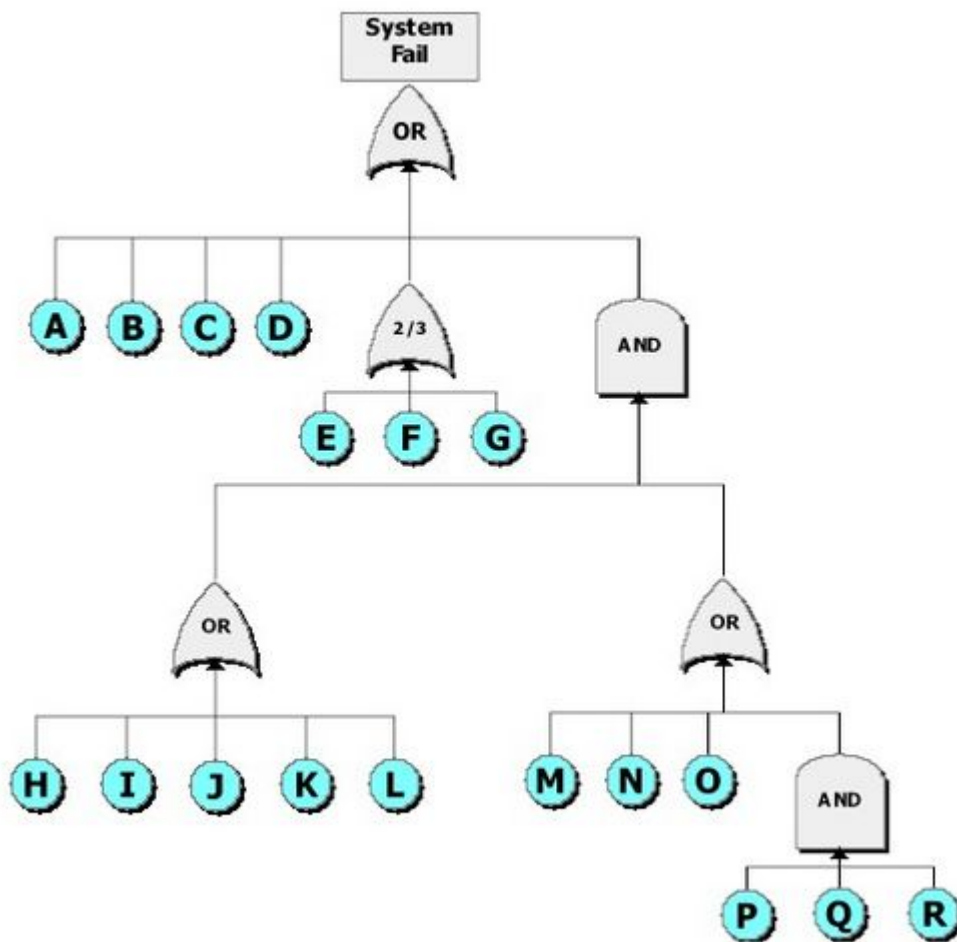
Figure 1. Fault Tree. (SEBoK Original)
