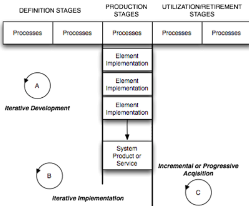
Figure 5. Iteration Through Life Cycle Stages (Lawson 2010).
