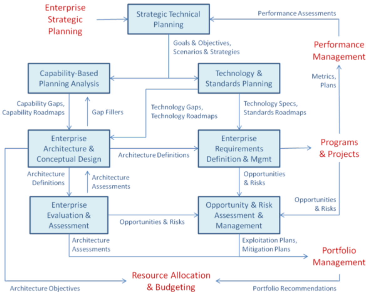
Figure 2. Enterprise Systems Engineering Process Activities. (SEBoK Original)
